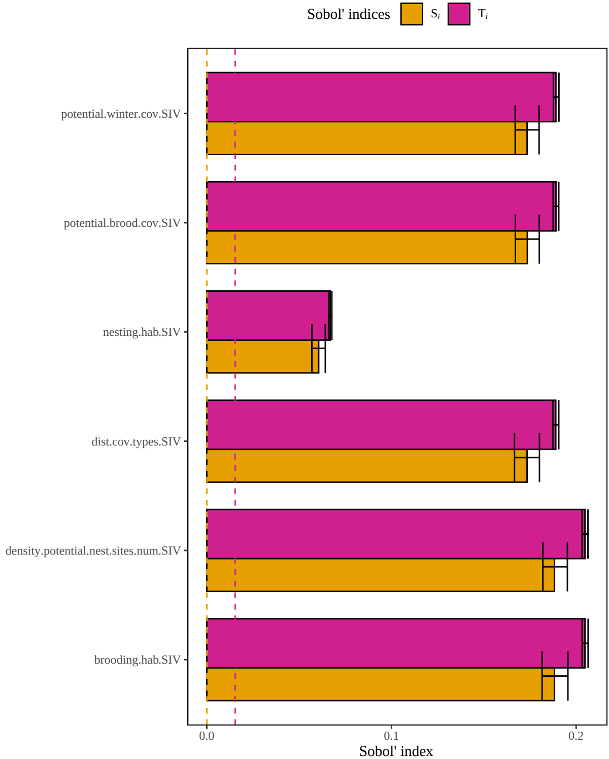
Figure 5. Results of a sensitivity analysis for the woodduckYear model based on a geometric mean structure. Dashed lines represent baseline numerical approximation error for S_i and T_i ( i.e. , dummy variables).
